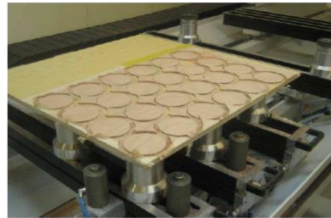
Figure 7: Cut of 24 circular specimens realized by means of a CNC milling cutter. Specimens were drilled and used for the Kundt's tube test
