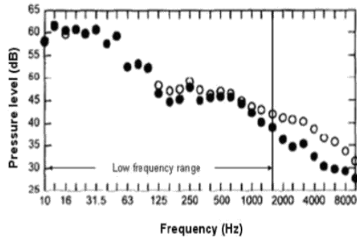
Figure 2: Example of noise spectra produced in an office with 24 workers: ○ within office hours; ● during lunch time (modified from [1])
