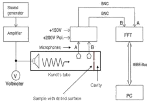
Figure 6: Outline of the test method device, mainly constituted by a sound generator, the Kundt's tube, two microphones, a FFT analyser and a PC for data processing
