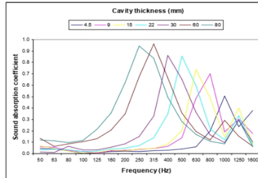
Figure 10: Sound absorption values measured for different cavity thickness
