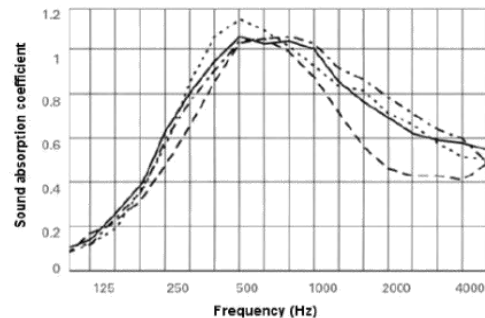
Figure 5: Sound absorption values of perforated wood-based panels with different passing light percentages: — (6.0%); ..... (7.0%); - · - · (7.5%); - - - (12.0%) [from 7]
