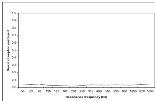
Figure 9: Sound absorption values measured for the undrilled plywood panel
