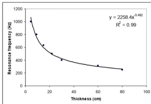
Figure 11: Cavity thickness vs. resonance frequency of the absorption peaks
