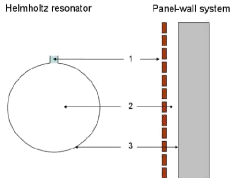
Figure 4: Longitudinal section of a Helmholtz resonator (left) and a system made of perforated panel and wall (right). 1 is the neck in the resonator, corresponding to the holes in the wood-based panel; 2 is the cavity, corresponding to the empty space between panel and wall; 3 is the cavity surface, which corresponds to the wall
