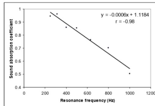
Figure 12: Negative linear correlation between resonance frequency and sound absorption coefficient achieved by the peaks
