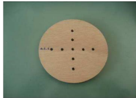
Figure 8: Tested specimen with diameter 99.8 mm and drilling pattern made of 9 holes of ray 2 mm symmetrically disposed
